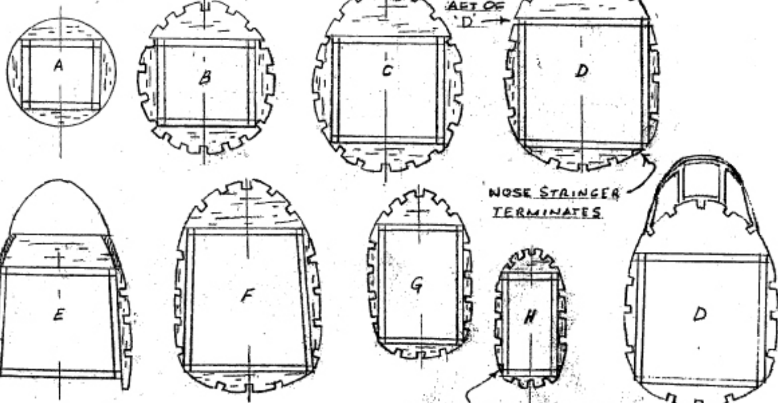
BOYANOWSKI P-39 FORMERS
