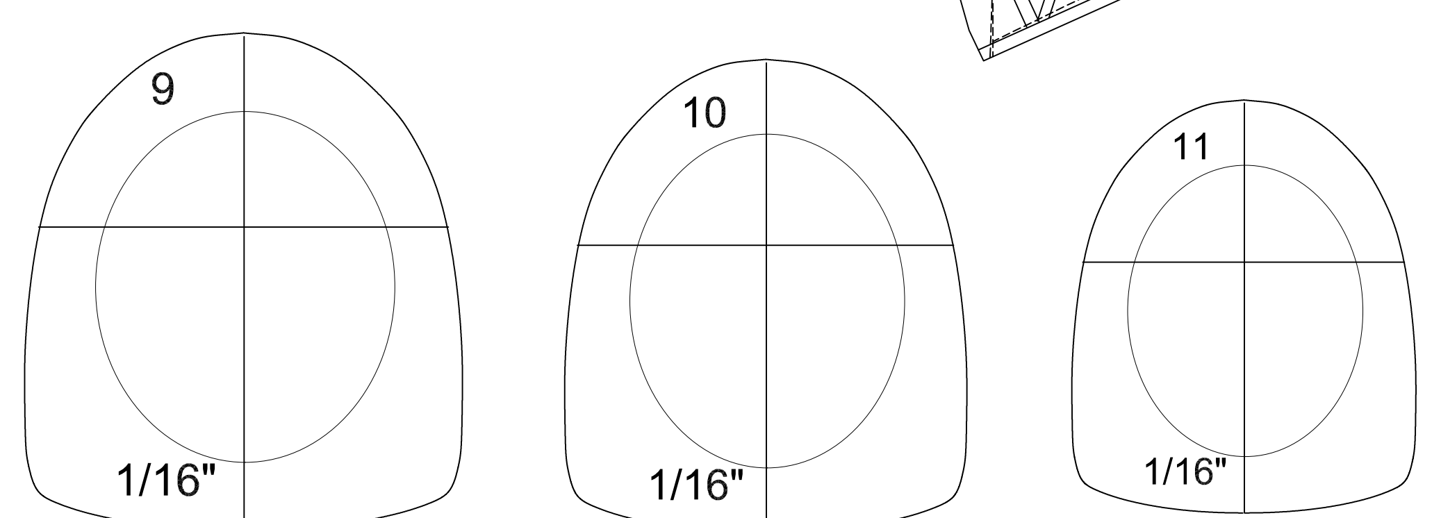
FUSELAGE FORMERS 1/16" SHEET
