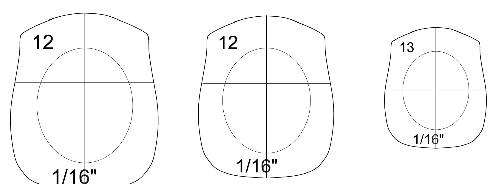
FUSELAGE FORMERS 1/16" SHEET
